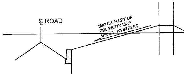
SMALL LOT / SMALL PROJECT IN CURB & GUTTER AREAS
