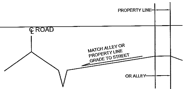
SMALL LOT / SMALL PROJECT IN OPEN CHANNEL AREAS
